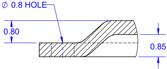
DETAIL A SCALE 12 : 10.8
