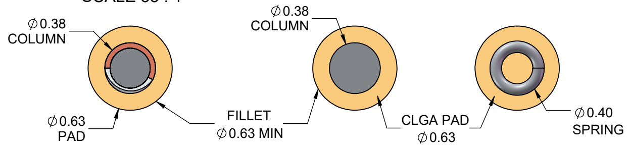
SECTION C-C SCALE 35 : 1
