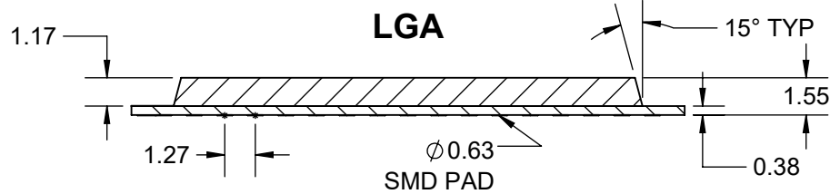
SECTION A-A SCALE 3.5 : 1
