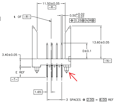
DETAIL Z SCALE 20:1
