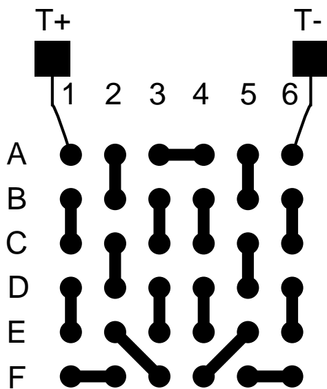
TEST VEHICLE BOARD
