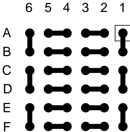
BALL VIEW
