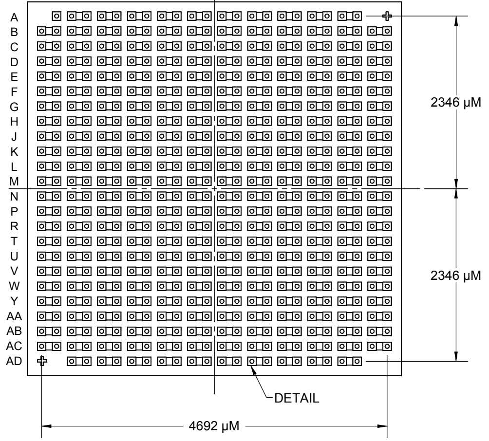
WIRE BONDING PAD DETAIL 2
