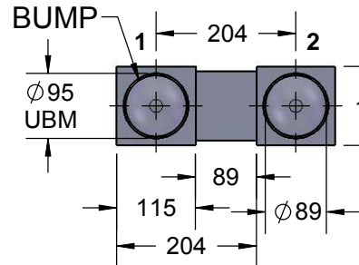
SOLDER BUMP PAD DETAIL 1
