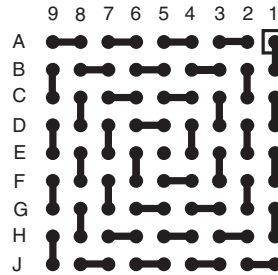
BGA81T.8-DC099
