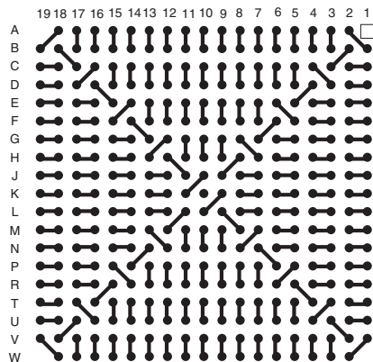
LBGA357T1.27-DC73
