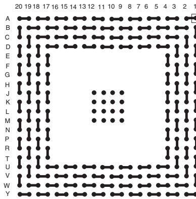
BGA272T1.27-DC202
