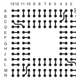
LBGA144T.8-DC134
