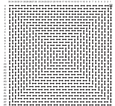
LBGA1225T1.27-DC359
