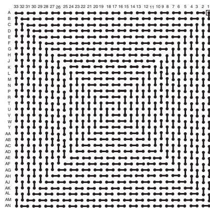
CBGA1089T1.27-DC339
