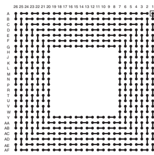
LBGA532T.8-DC266
