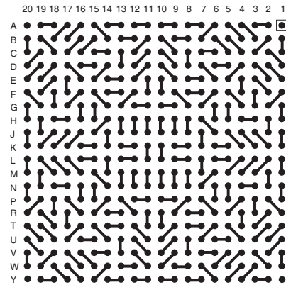
CBGA400T1.27-DC21
