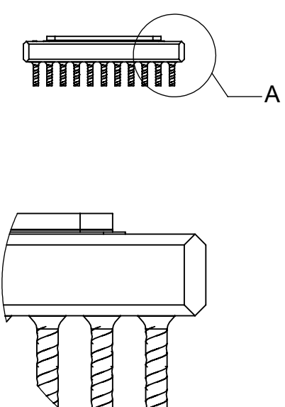
DETAIL A SCALE 8 : 1
