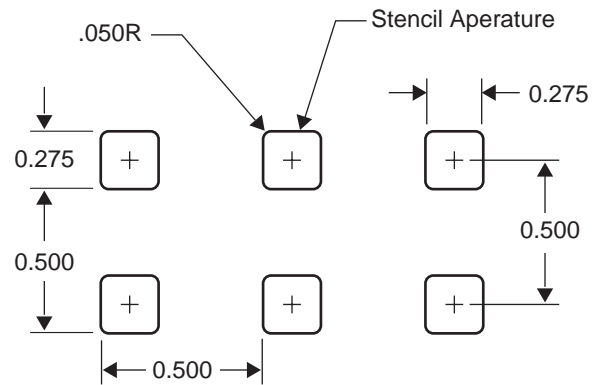
RECOMMENDED STENCIL
