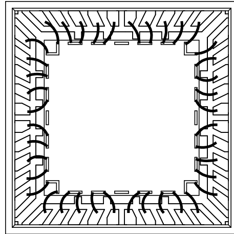
QFN40W.5-DCW40402 40L - 6X6mm
