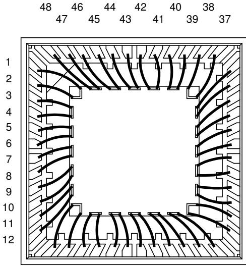
13 15 17 19 21 23 14 16 18 20 22 24 QFN48W.5-DCW40481 48L - 7X7mm
