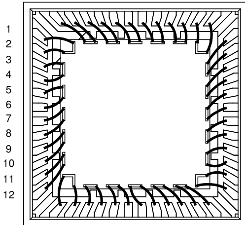
QFN48W.4-DCW40481 48L - 6X6mm
