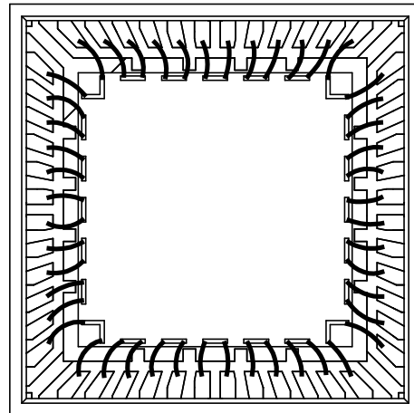
QFN48W.4-DCW40482 48L - 6X6mm
