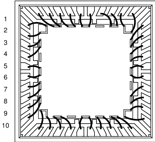
QFN40W.5-DCW40401 40L - 6X6mm
