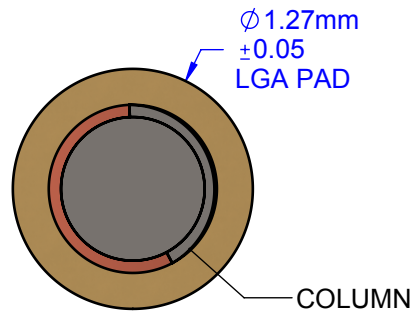
LGA - LAND GRID ARRAY PAD PLATING Ni-Au
