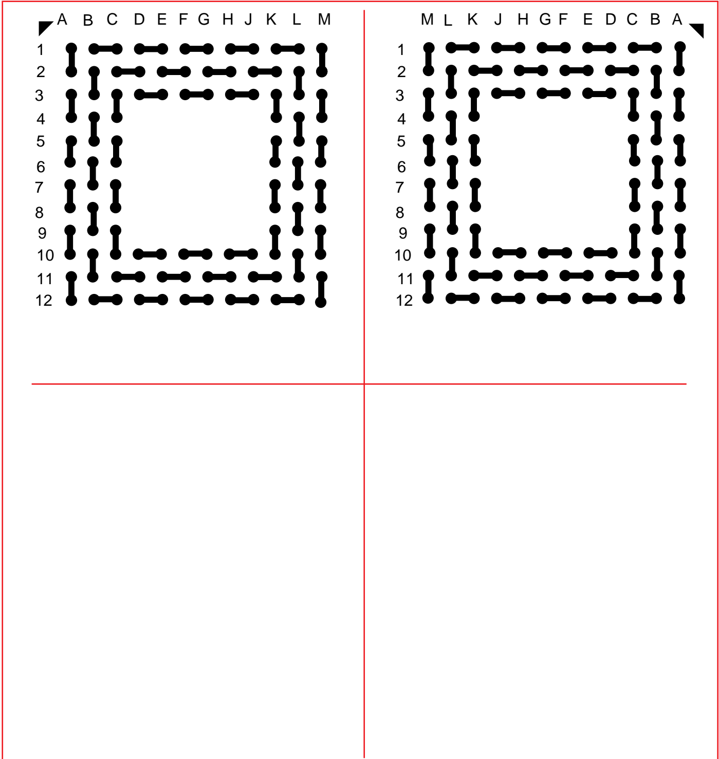
BOTTOM SIDE (TOP X-RAY VIEW)
