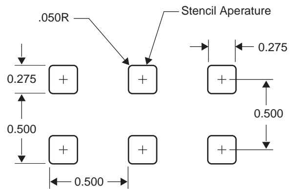
RECOMMENDED STENCIL
