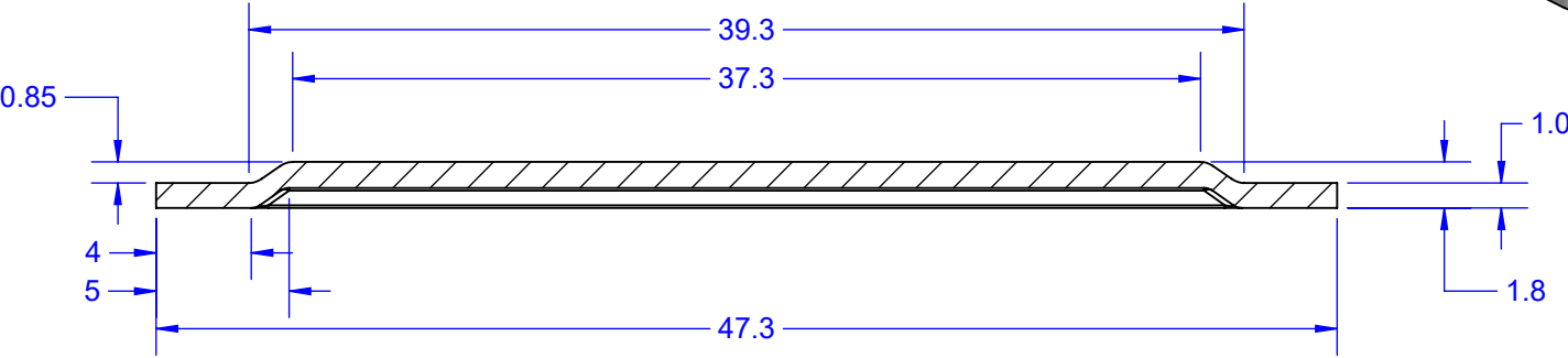
SECTION B-B
