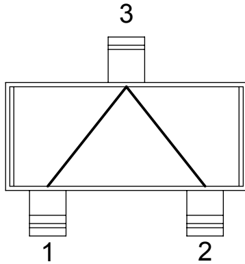
SOT23 - DC123 SOT323 - DC123 DWG 120123
