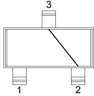
SOT23 - DC23 SOT323 - DC23 DWG 123023
