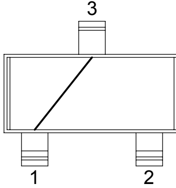
SOT23 - DC13 SOT323 - DC13 DWG 120313
