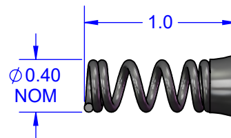
MICRO-COIL SPRING
