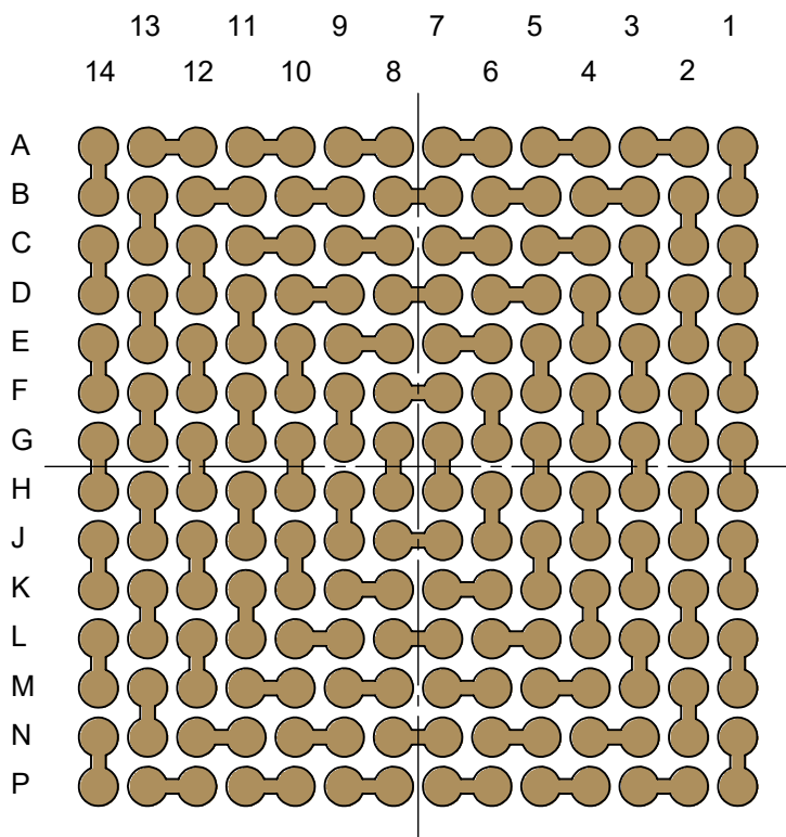
COLUMN (PAD) VIEW
