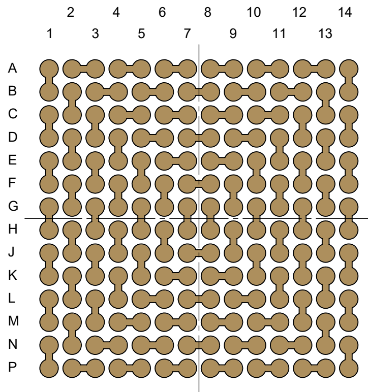
BOTTOM X-RAY VIEWED FROM TOP
