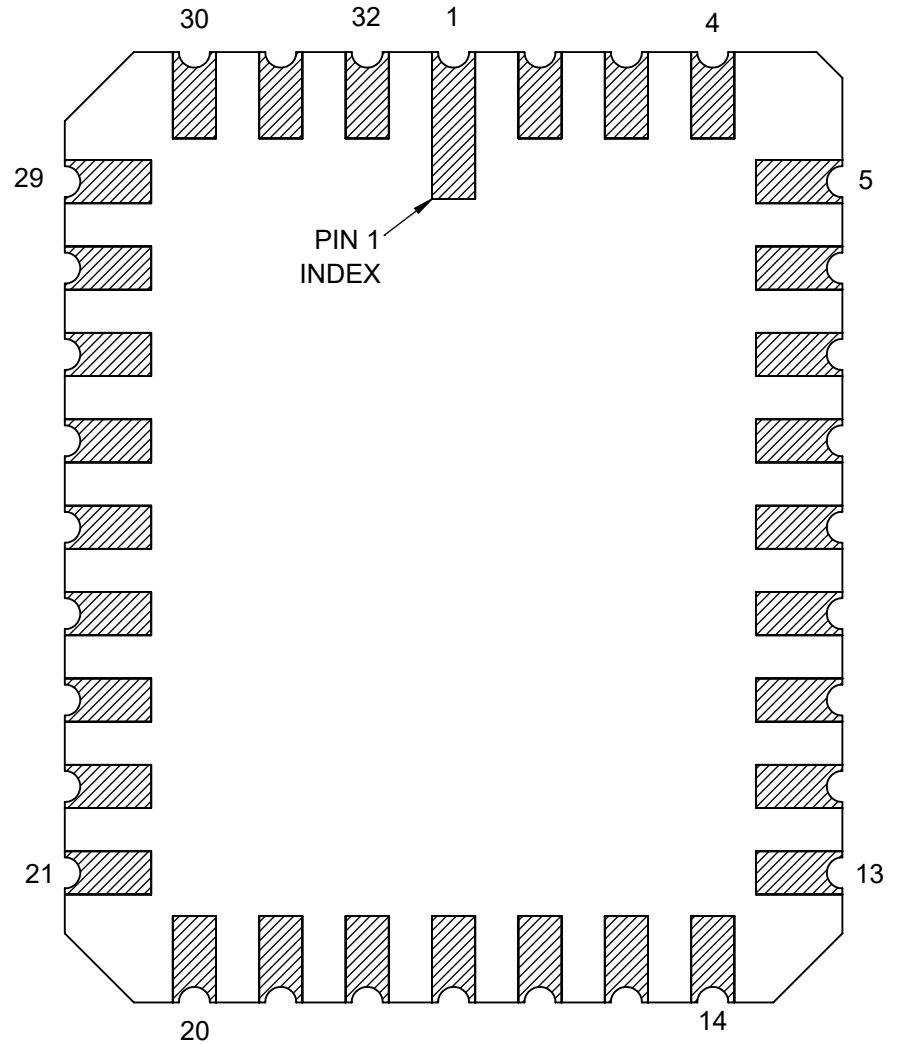
BOTTOM VIEW
