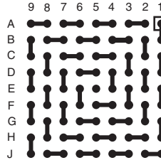
BGA81T.8-DC099
