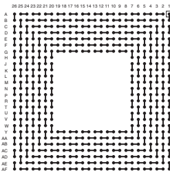
LBGA532T.8-DC266
