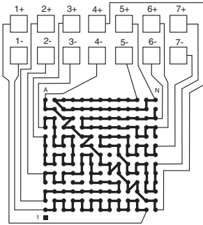
BGA169 AFTER MOUNTING TO TEST BOARD
