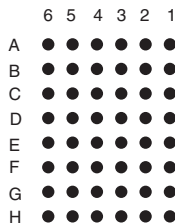
BGA48T.75-6x8
