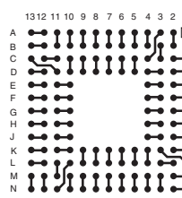
LBGA144T.8-DC134
