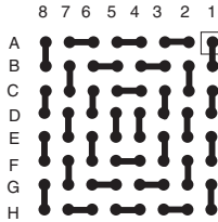
LBGA64T.8-DC089
