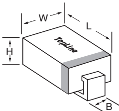
J-LEAD
