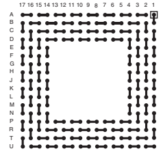
LBGA208T.8-DC170
