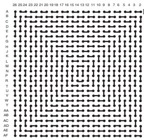
LBGA676T.8-DC269
