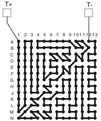
BGA169 AFTER MOUNTING
