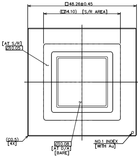
DIE PAD 0.840" x 0.840" 21.24 x 21.24mm
