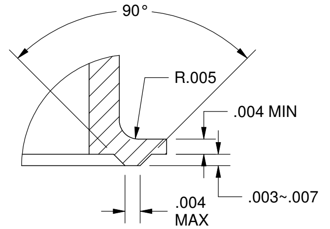
DETAIL A SCALE 40 : 1
