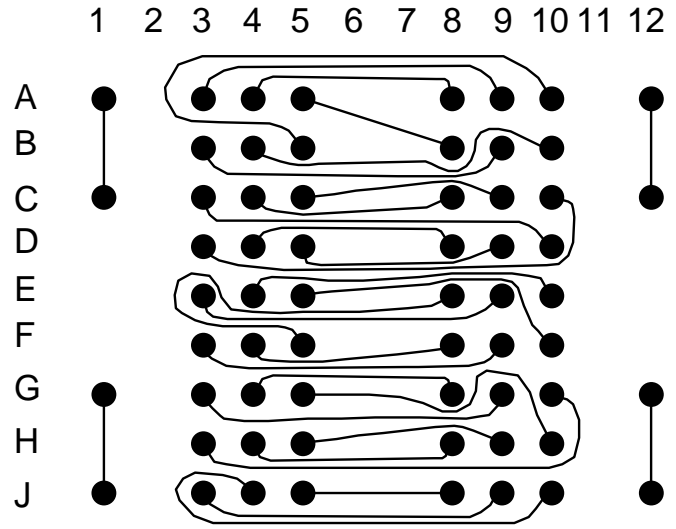
BOTTOM SIDE (TOP X-RAY VIEW)
