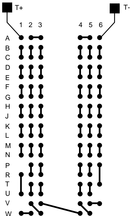
TEST VEHICLE BOARD
