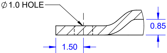
DETAIL E SCALE 8 : 1
