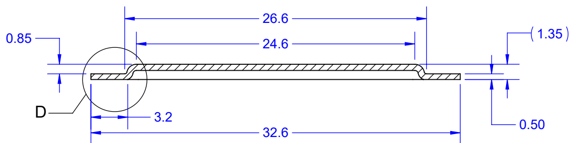
SECTION C-C SCALE 3 : 1
