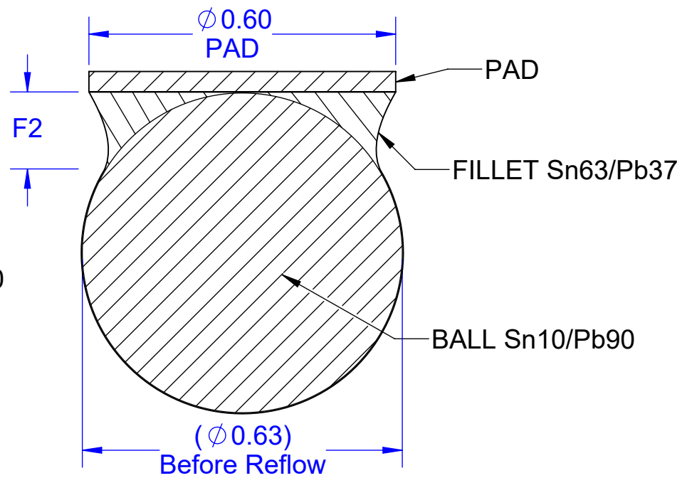
OPTION B SECTION VIEW
