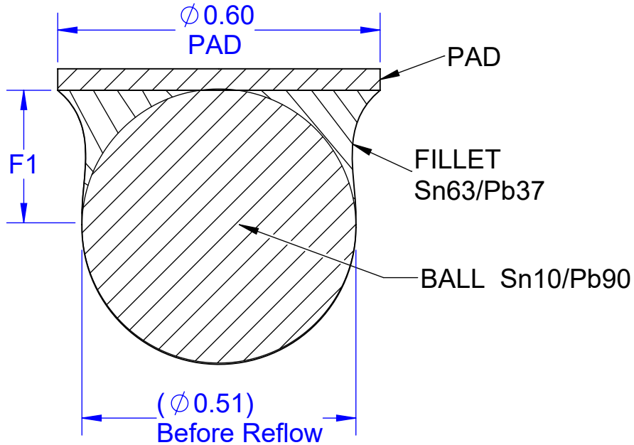
OPTION A SECTION VIEW
