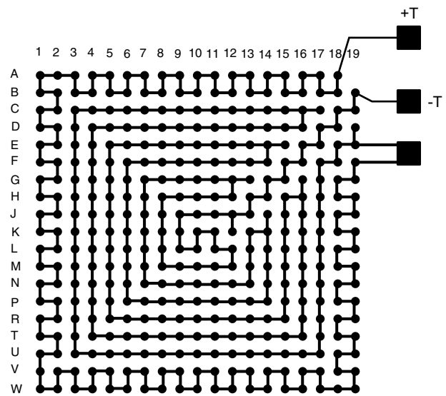
AFTER MOUNTING TO TEST BOARD
