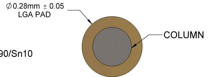
LGA - LAND GRID ARRAY PAD PLATING Ni-Au
