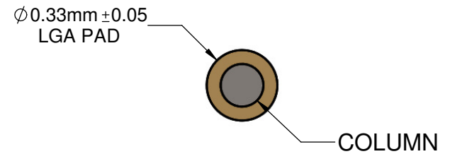
LGA - LAND GRID ARRAY PAD PLATING Ni-Au
