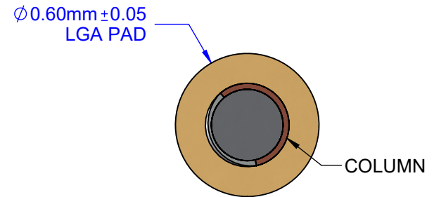
LGA - LAND GRID ARRAY PAD PLATING Ni-Au
