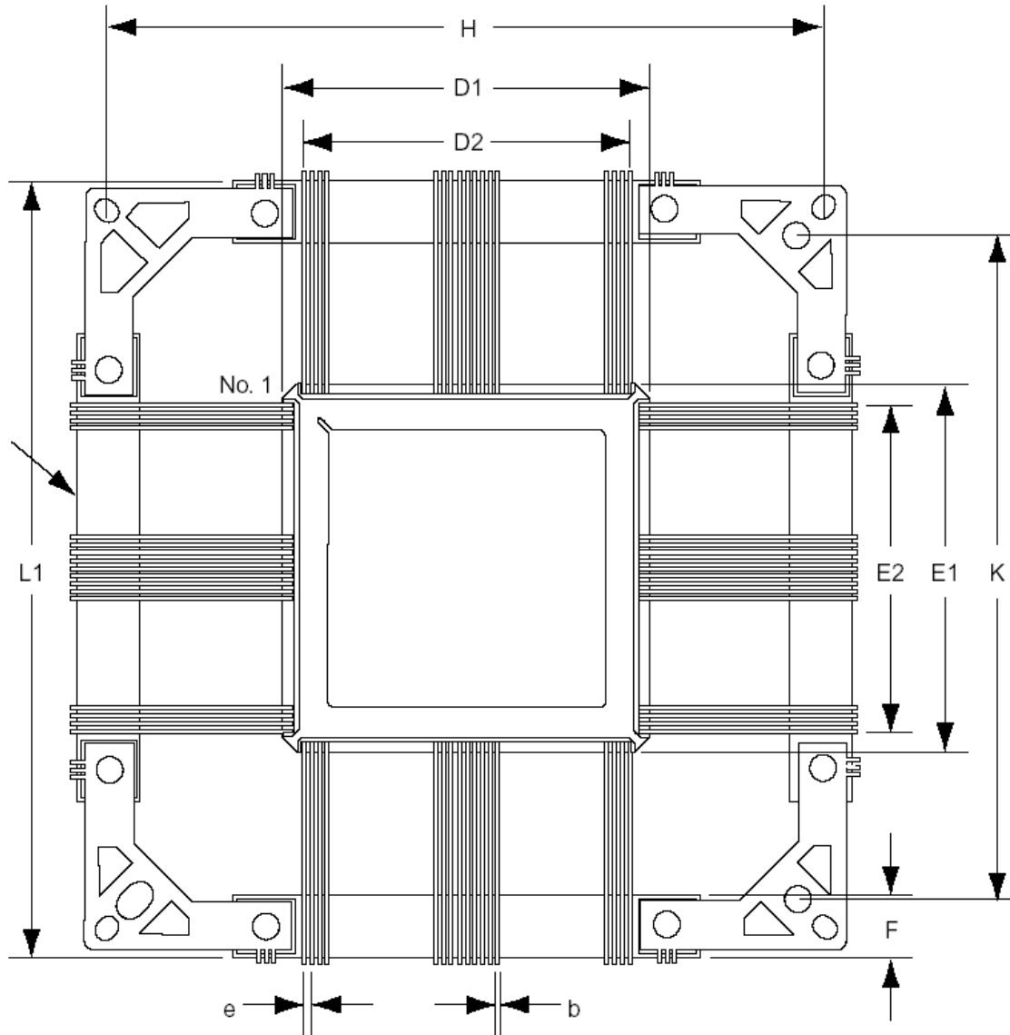
Top View
