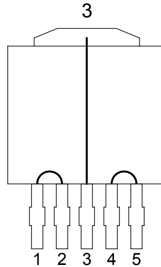
D2PAK5 - DC1245 DWG 121245
