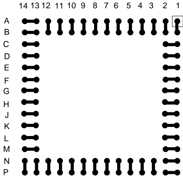
Pad VIEW
