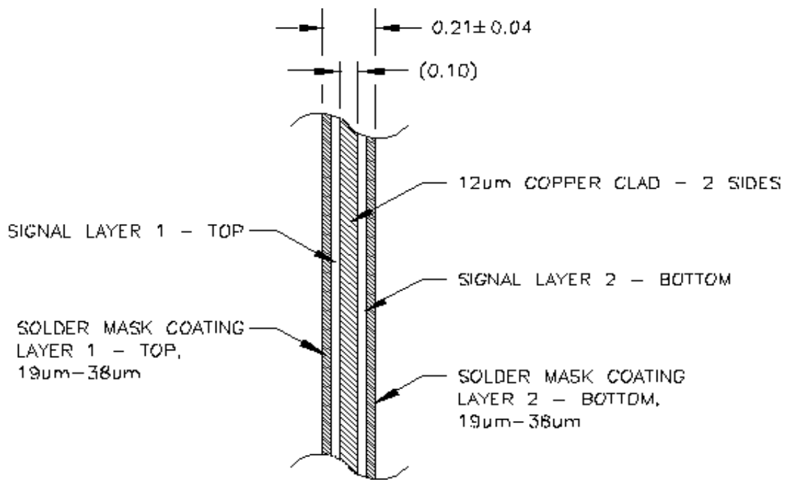
CROSS SECTION
