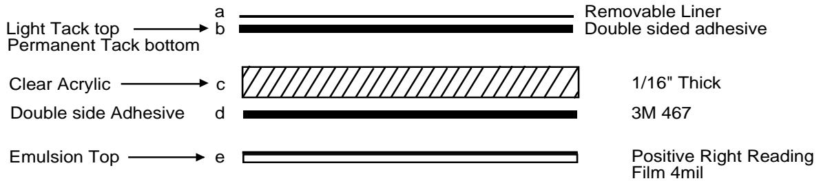
Side View (Not to Scale)
