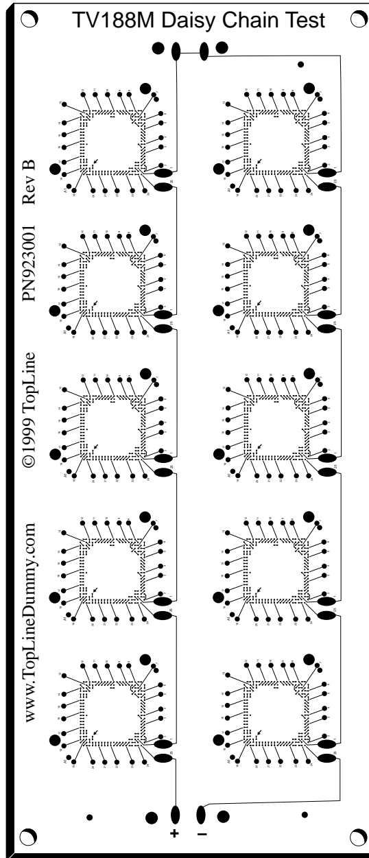
Component - Top (Metalization Layer)
