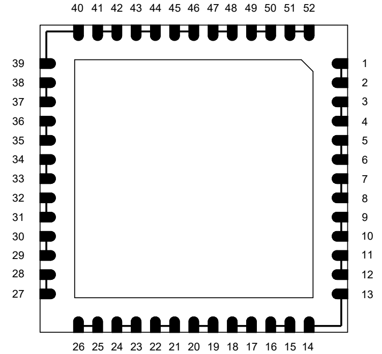
BOTTOM VIEW
