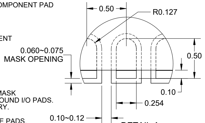
DETAIL A SCALE 40 : 1
