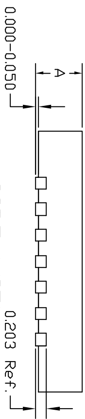
SIDE VIEW
