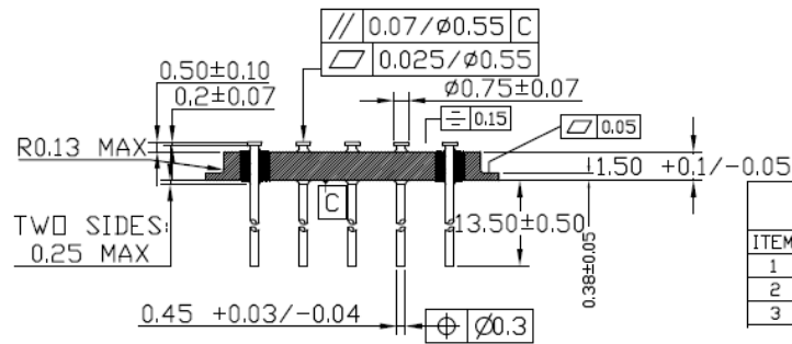
SECTION A-A SIDE VIEW
