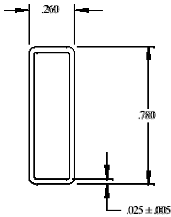
PLCC44 Tube
