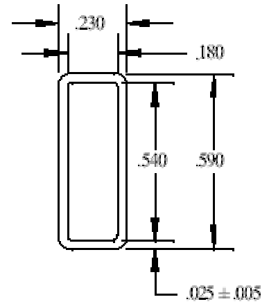
PLCC32 Tube
