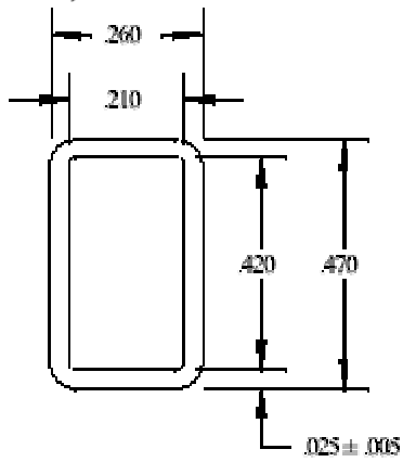
PLCC20 Tube
