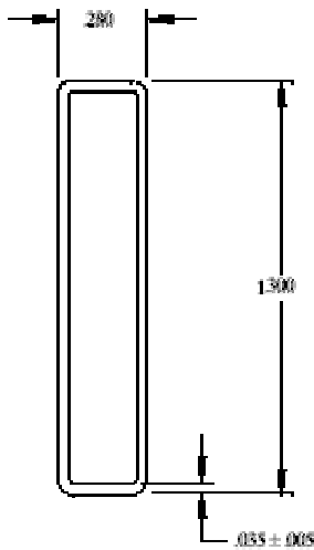
PLCC84 Tube
