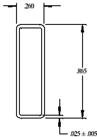
PLCC52 Tube
