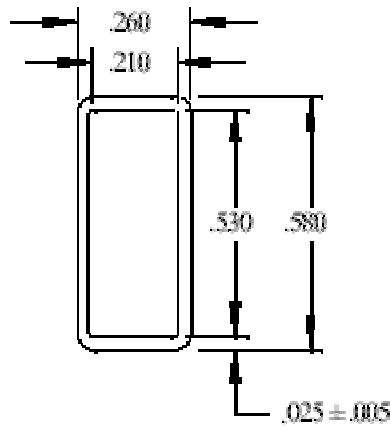
PLCC28 Tube
