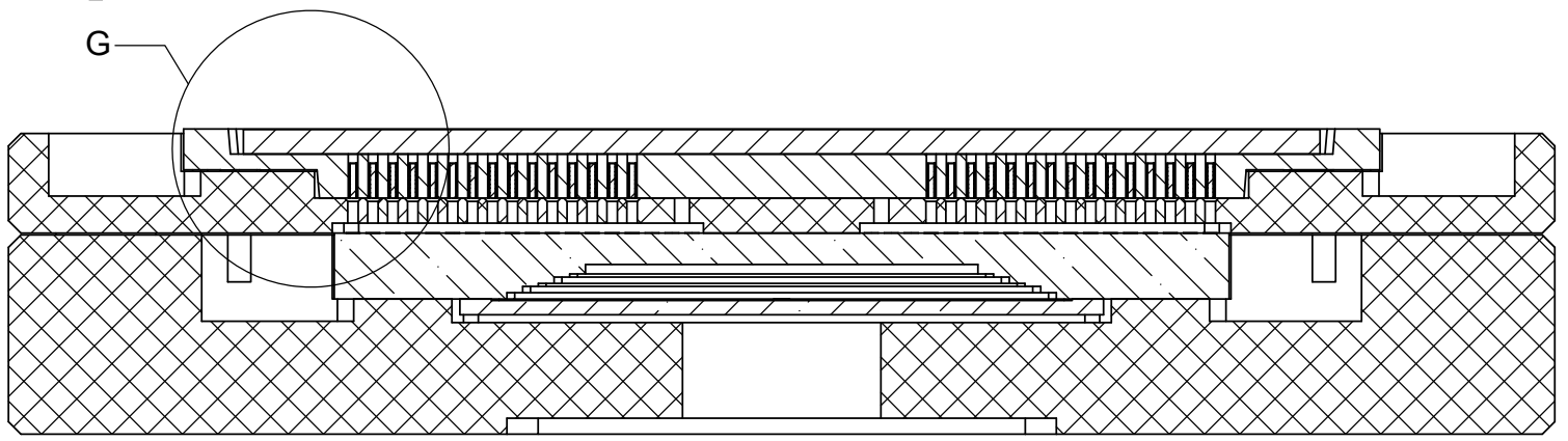
SECTION F-F SCALE 2 : 1
