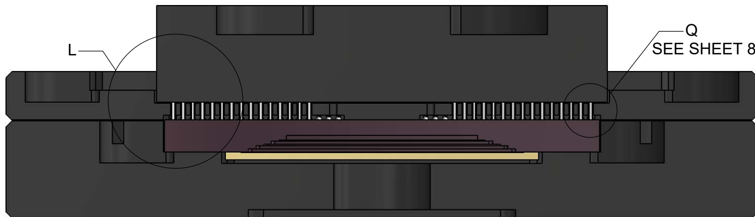
SECTION K-K SCALE 2 : 1
