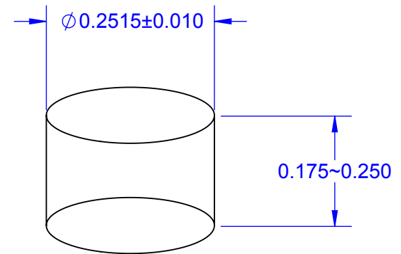
MOUNTING HOLE REMOVABLE PEG
