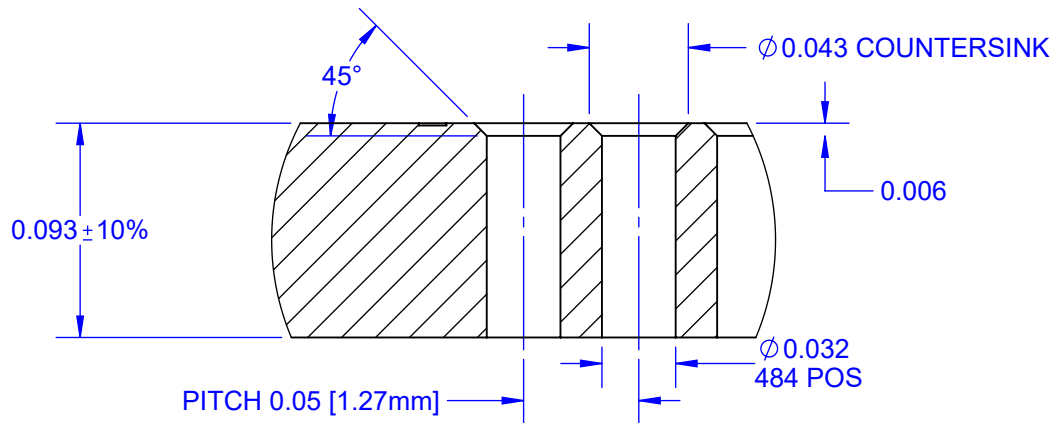
DETAIL B
