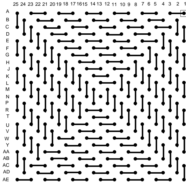
BALL VIEW
