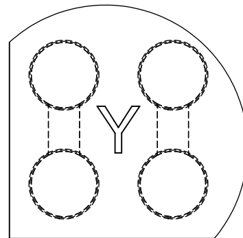
DAISY CHAIN ORIENTATION DETAIL B SCALE 60 : 1
