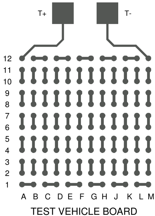
TOP VIEW
