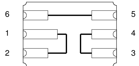
DAISY CHAIN (OPTIONAL) VIEWED FROM TOP
