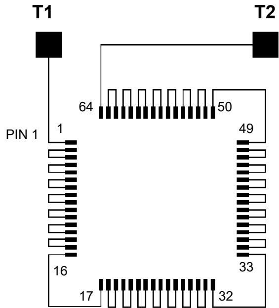
PCB PADS
