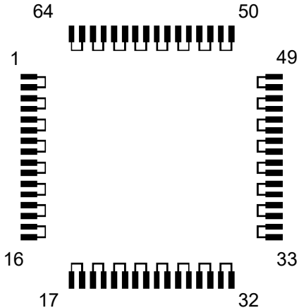
TOP COMPONENT
