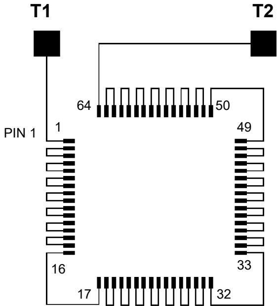
PCB PADS
