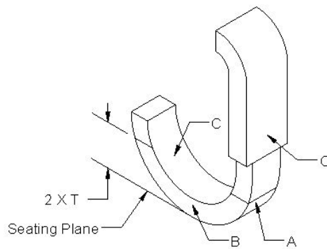
FIGURE 2003-6. Critical area for J-lead devices. Critical area = "A" (equal to 2x Lead Thickness) and edges "B" within the 2xT zone. Surface "C" is excluded.
