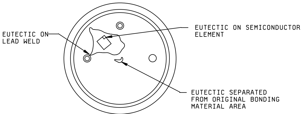
FIGURE 2012-10. Acceptable and unacceptable excess material.
