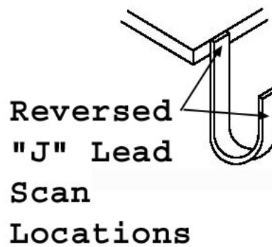
FIGURE 2037-4. Scan Locations on Reversed J-Style lead.
