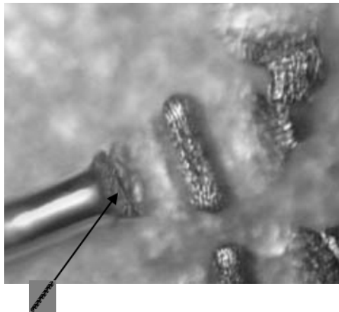
Reject bond is cracked at the heel. Figure 2017-20e.
